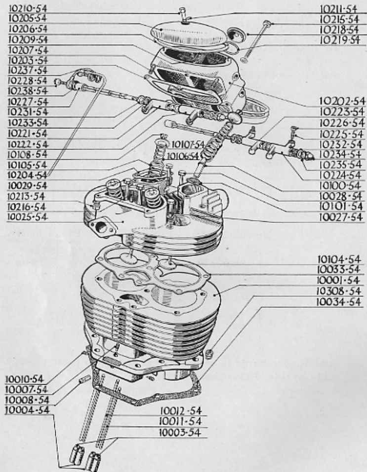
ARIEL 650 c.c. TWIN CYLINDER HUNTMASTER
