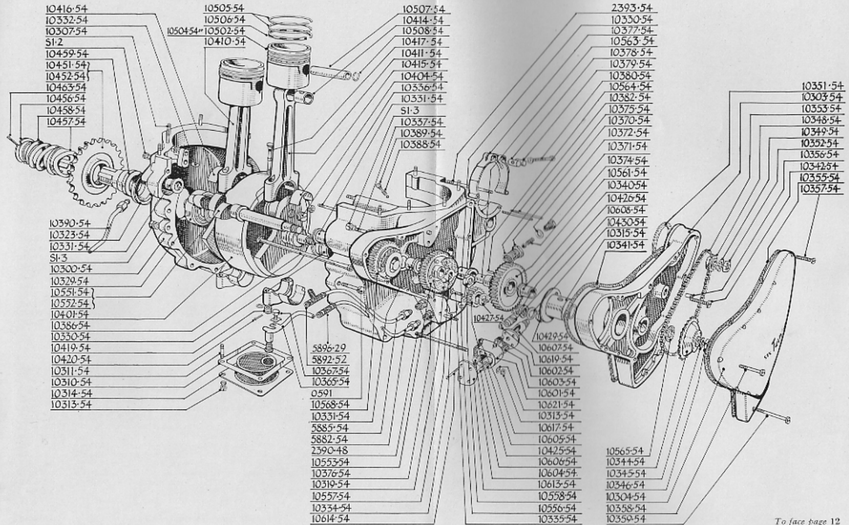
ARIEL 650 c.c. TWIN CYLINDER HUNTMASER
