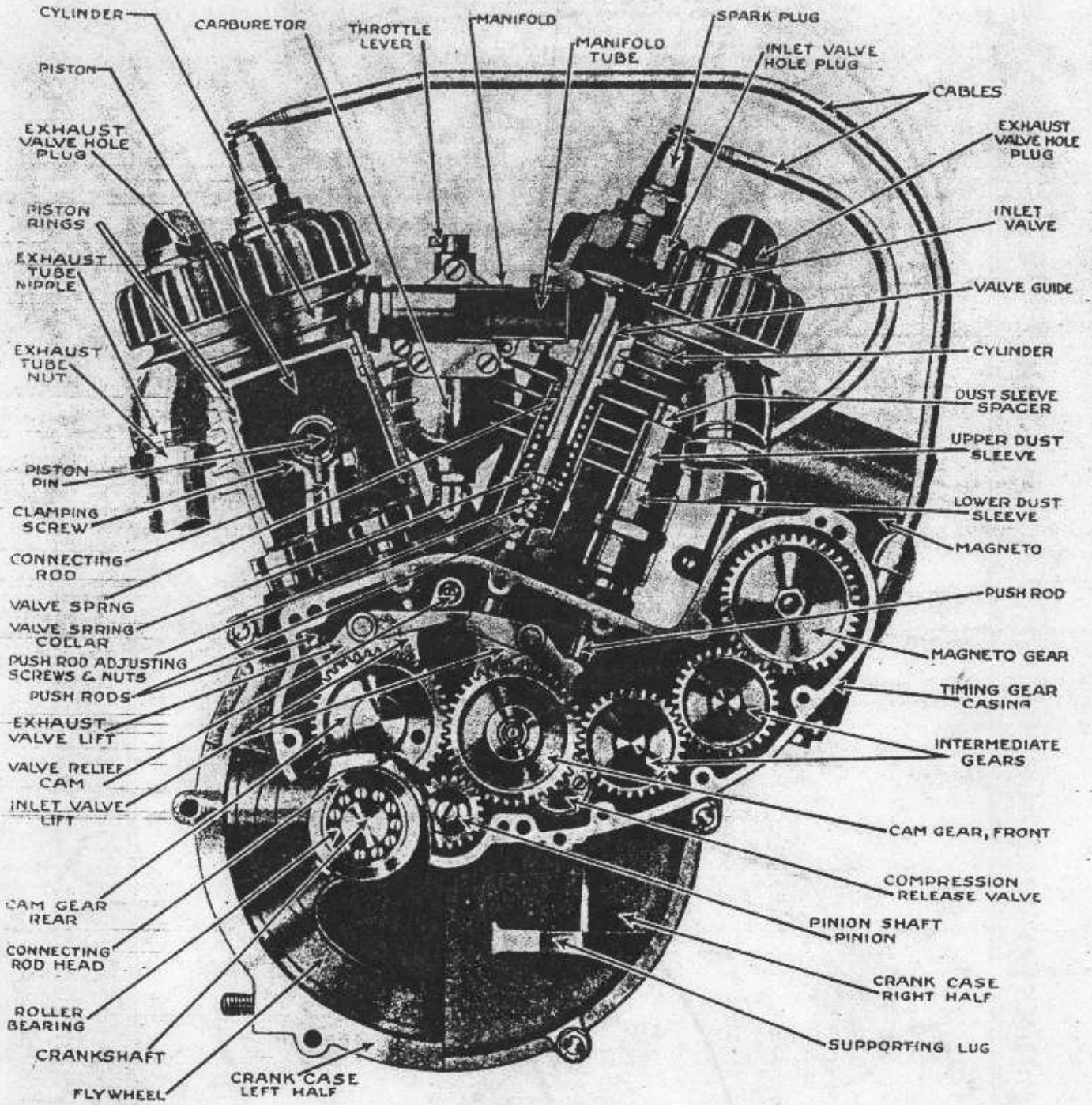
Sectional View G-20 Motor
