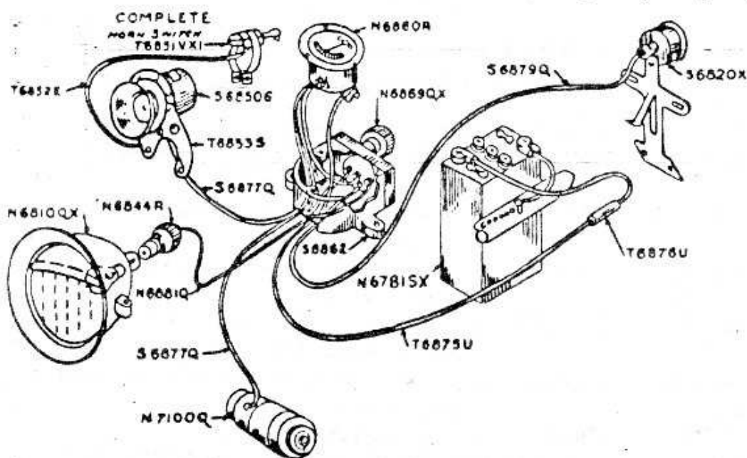
Wiring Diagram 1926
